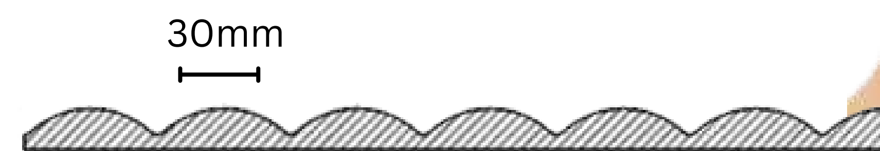
FLEXIBOARD CURVED OUT
